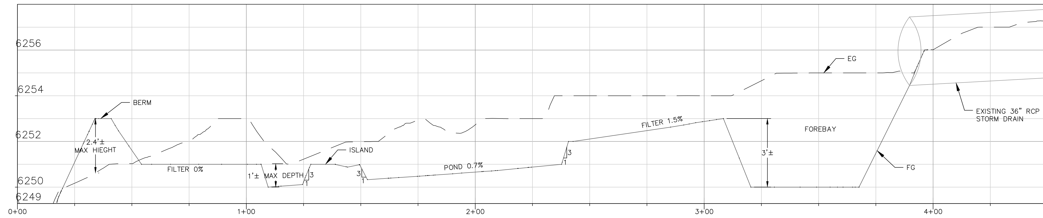
PROFILE HORIZ SCALE 1"=20', VERT SCALE 1" = 2'
