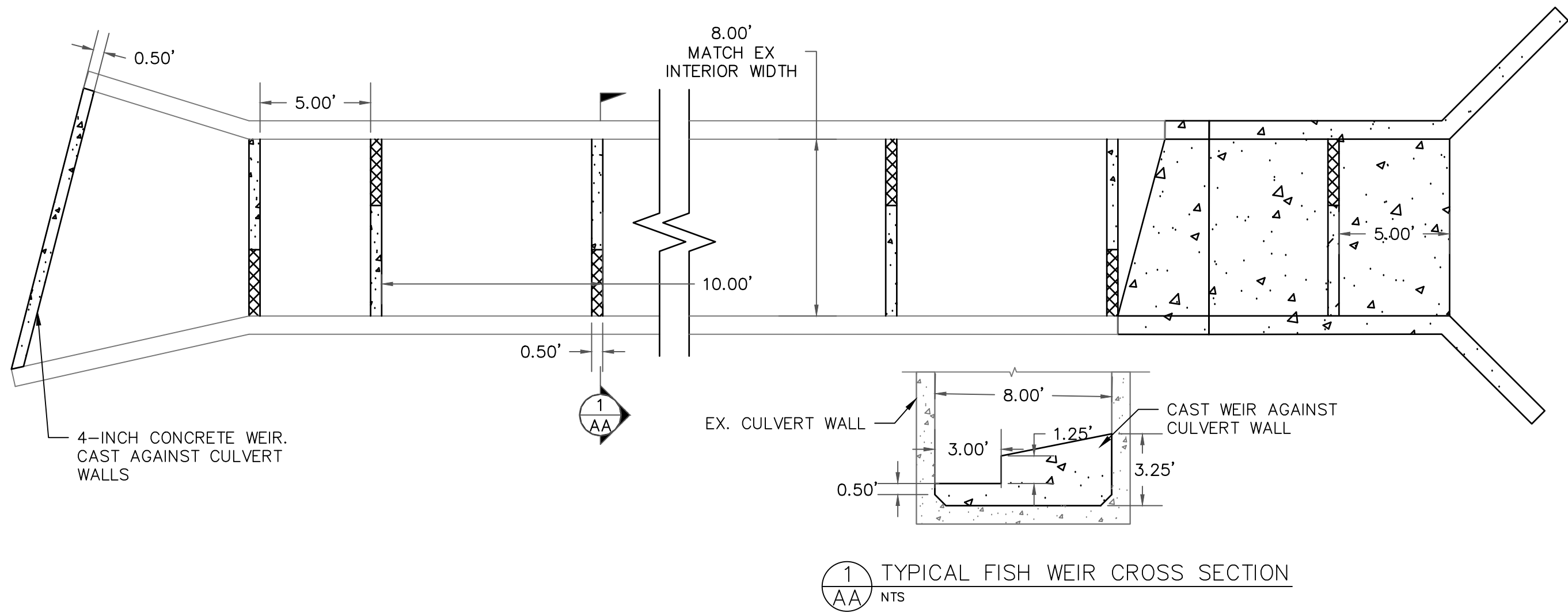
1 D5 NTS CULVERT FISH WEIR LAYOUT
