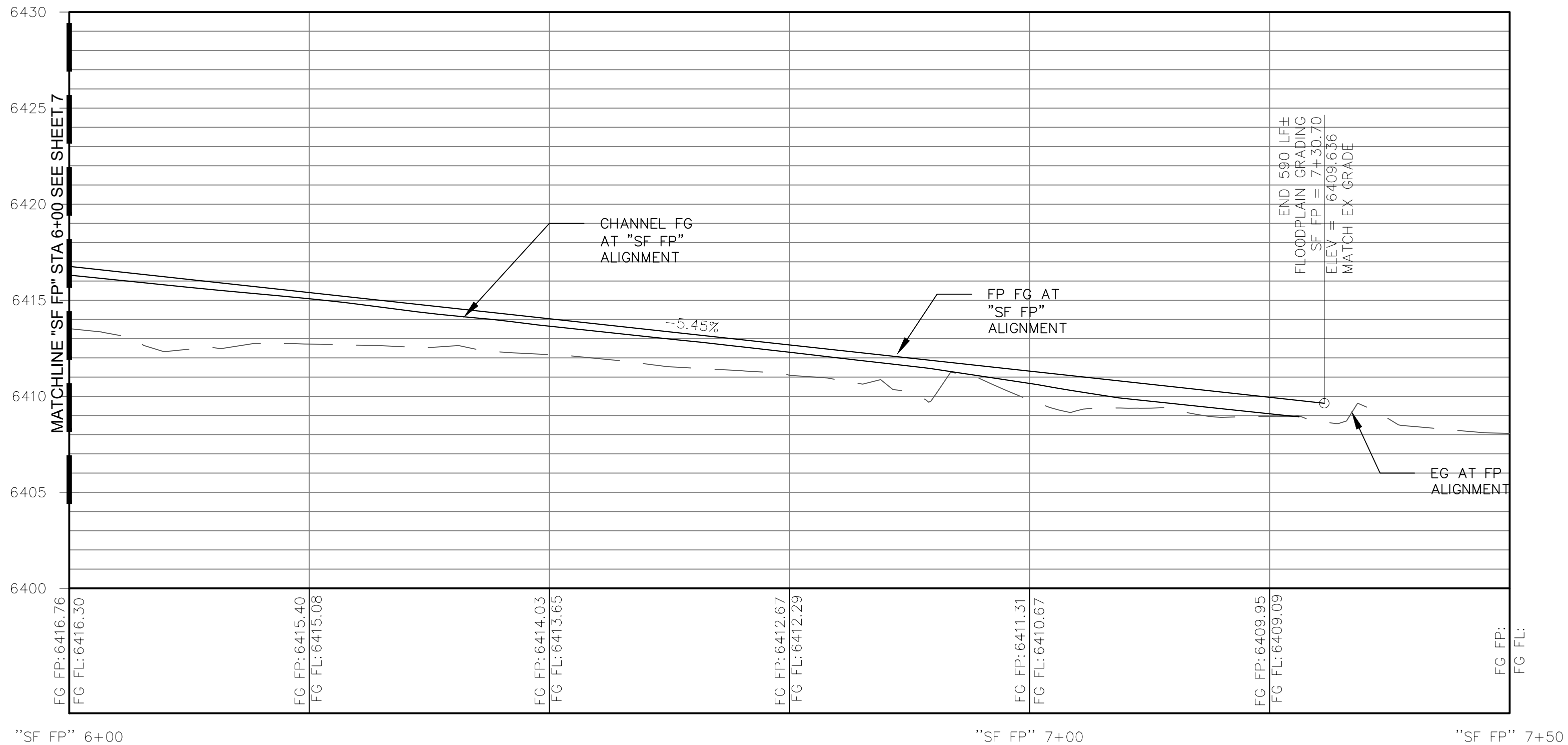
"SF-FP" PROFILE
