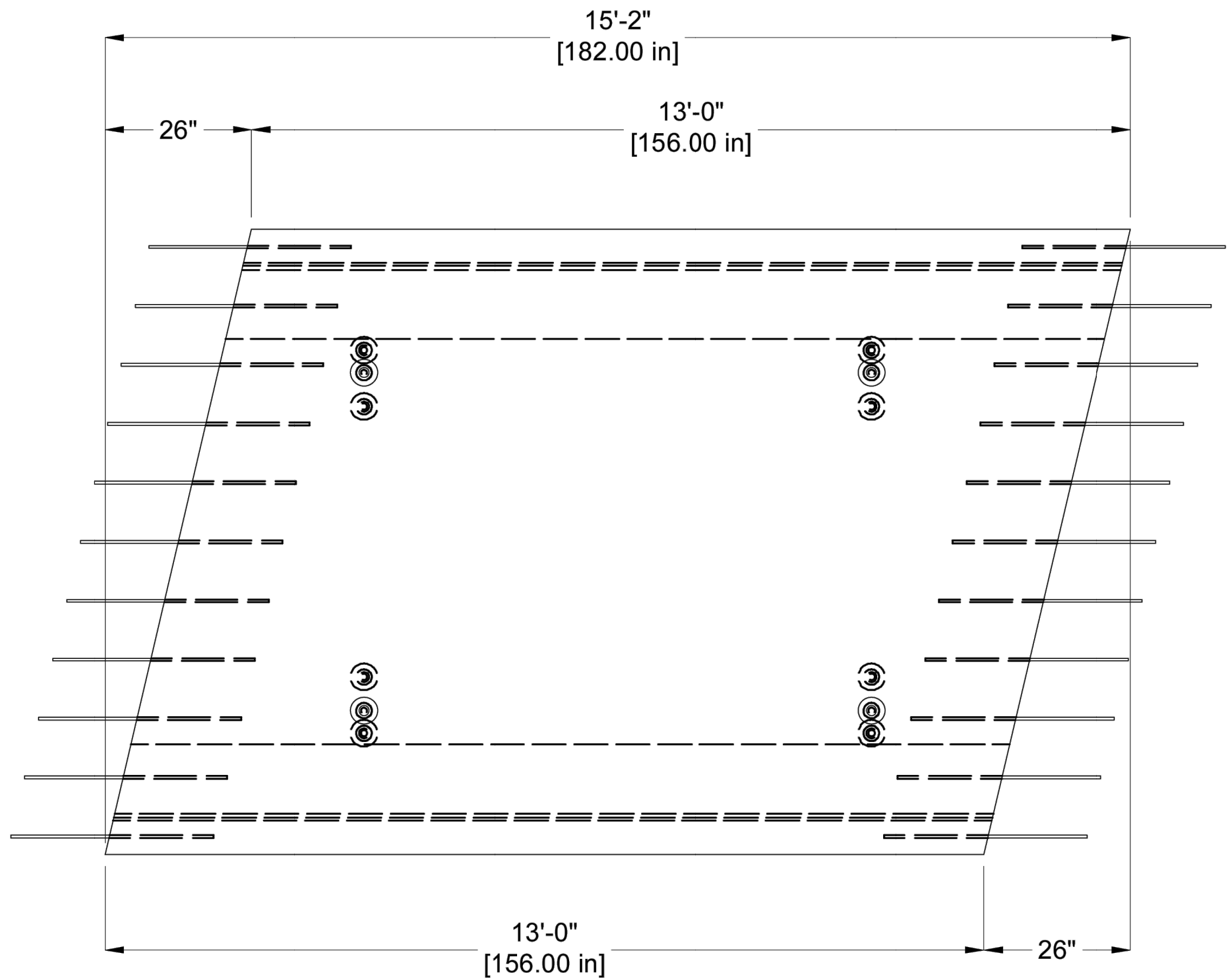
PLAN VIEW
