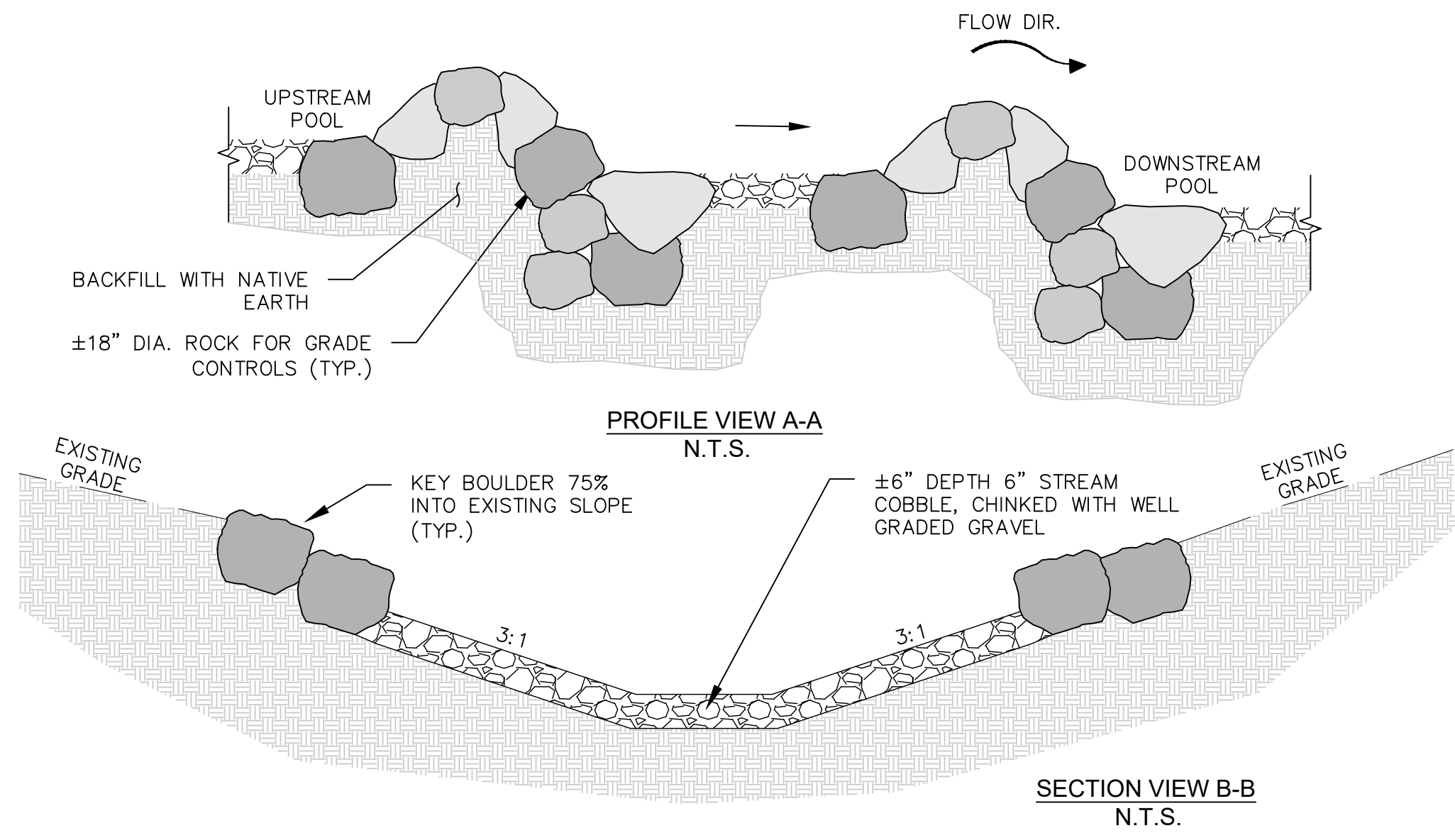
3 D5 NTS SOUTH FORK BOULDER GRADE CONTROL
