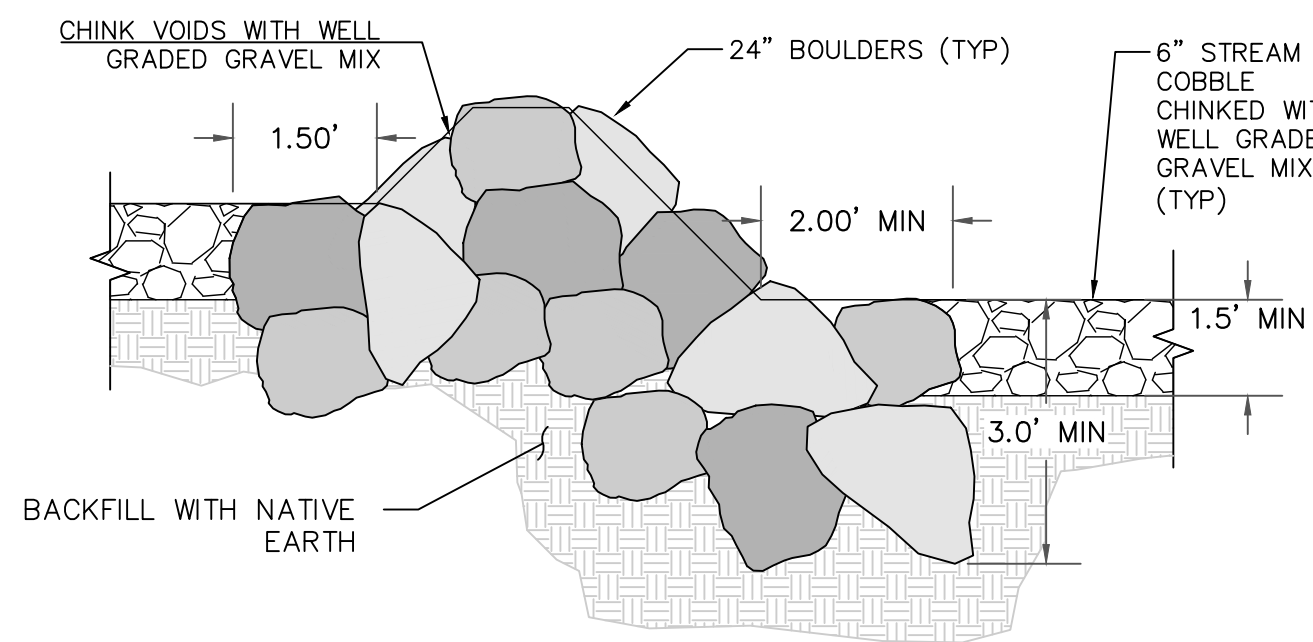
2 D5 NTS MAIN FORK BOULDER GRADE CONTROL
